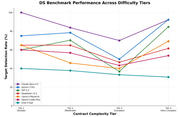
Figure 6: DS performance across difficulty tiers. Performance generally falls on harder contracts, although the pattern is not monotonic for every model. Tier 4 contains 13 expert-level contracts, so its rates should be read with this smaller sample size in mind.
