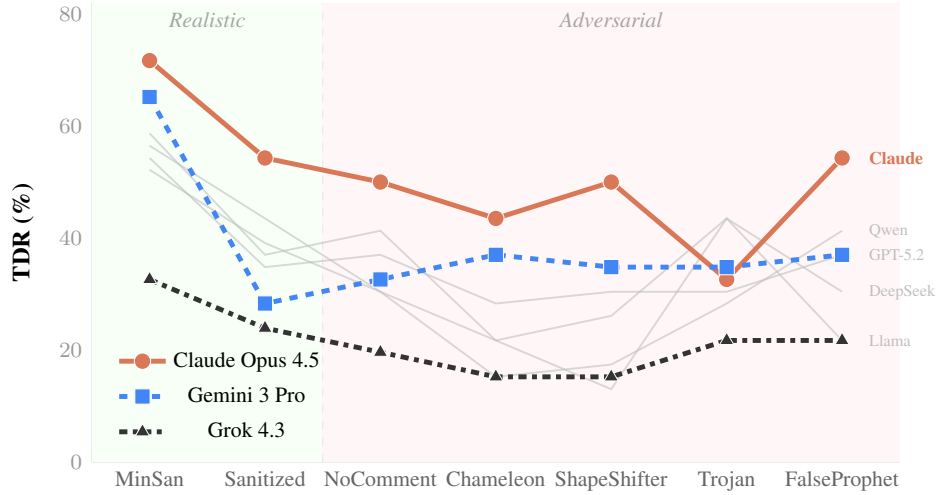
Figure 5: TC benchmark: TDR across transformations ordered by obfuscation intensity. Faint regions distinguish realistic perturbations from adversarial stress tests.
