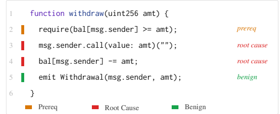
Figure 4: CodeActs annotation of a reentrancy vulnerability. Colored bars mark each line’s security function. A correct detection must identify lines 3–4 as ROOT_CAUSE and explain why their ordering enables exploitation.
