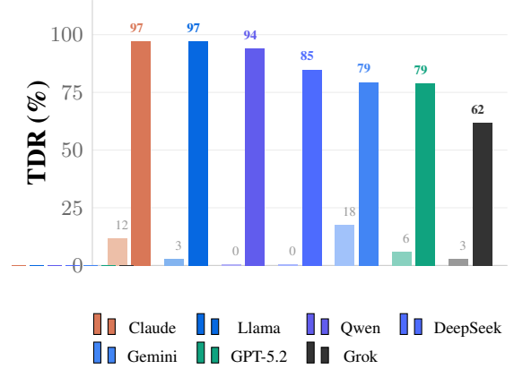
Figure 1: Temporal gradient in GS performance. Light bars show samples with 2–6 months of public exposure and an average TDR of 5.9%. Dark bars show samples with 7–8 months of exposure and an average TDR of 84.7%. Detection rises with exposure. This is consistent with possible contamination but does not prove its cause. On the most recently disclosed samples ( n=72 ), average TDR remains at 0.8%.
