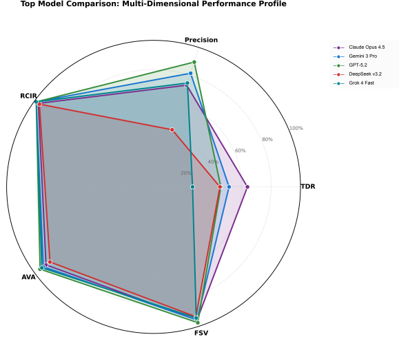
Figure 8: Performance profiles for five selected models across Target Detection Rate (TDR), Finding Precision, Root Cause Identification (RCIR), Attack Vector Accuracy (AVA), and Fix Suggestion Validity (FSV). Claude Opus 4.5 shows a balanced profile with the highest TDR, while GPT-5.2 has the highest precision at 89.6%.
