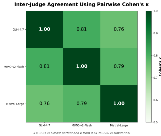
Figure 7: Pairwise agreement among the three judges used for DS and TC. All pairs achieve substantial agreement ( \kappa \geq 0.76 ). On GS, the two primary judges, GLM-4.7 and MIMO-v2-Flash, achieve \kappa = 0.943 with 97.7% agreement.
