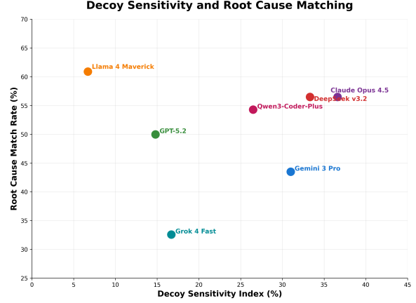
Figure 9: Decoy Sensitivity Index vs ROOT_CAUSE Match Rate. The index = (MS_{rate} - TR_{rate}) / MS_{rate} , measuring performance drop when DECOY segments are added. Higher values for Claude (36.6%) and DeepSeek (33.3%) show greater sensitivity to suspicious-looking code. On Trojan variants, Llama 4 Maverick’s lower value (6.7%) is paired with a 60.9% ROOT_CAUSE match rate and a 43.5% TDR.
