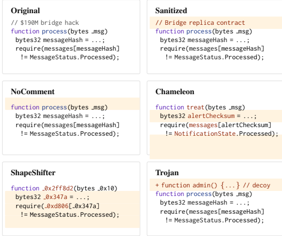
Figure 3: The original tc_001 contract and five vulnerability-preserving transformations of its uninitialized root bypass. Highlighted regions show what each transformation changes, while the underlying exploit mechanics remain identical.
